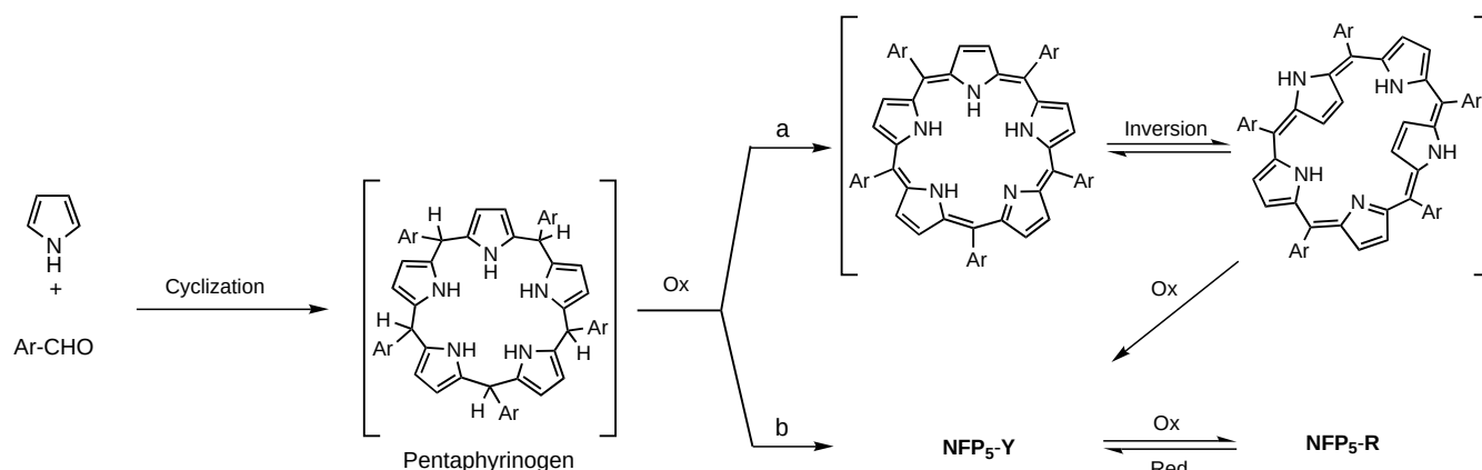
Scheme 2. A possible reaction mechanism for the formation of \text{NFP}_5 .
